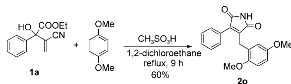
Scheme 3. Synthesis of 3,4-disubstituted maleimide derivatives by the reaction of 1a with 1,4-dimethoxybenzene.
