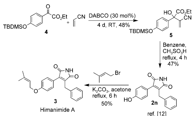
Scheme 2. Simple route for the synthesis of 3 . [11] DABCO = 1,4-diazabicyclo[2.2.2]octane, TBDMS = tert -butyldimethylsilyl.
