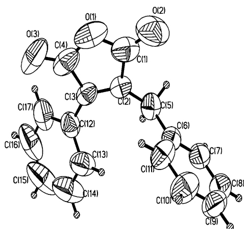
Figure 2. ORTEP diagrams of compounds 2k and 7a . Ellipsoids at 50% probability.
